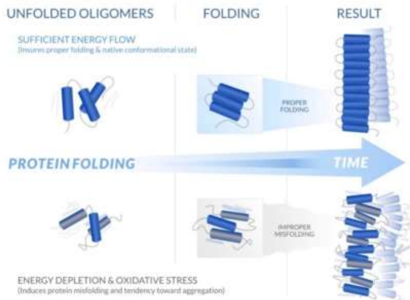
Figure 1 Proper 3D conformation of a protein is dependent on available energy in the cellular
